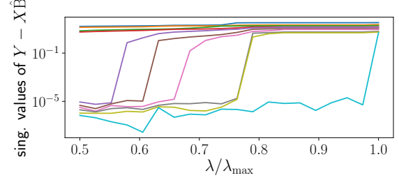
Figure 2: Singular values of the residuals Y - X\hat{B} of the multivariate square-root Lasso ( n = 10, q = 20, p = 30 ), as a function of \lambda . The observation matrix Y is full rank, but the residuals are rank deficient even for high values of the regularization parameter, invalidating the classical assumptions needed for statistical analysis.
