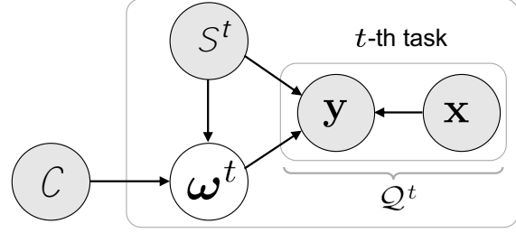
Figure 2. Illustration of MetaVRF in a directed graphical model, where (\mathbf{x}, \mathbf{y}) is a sample in the query set \mathcal{Q}^t . The base \mathbf{!}^t of the t -th task is dependent on the support set S^t of the current task and the context \mathcal{C} of related tasks.
