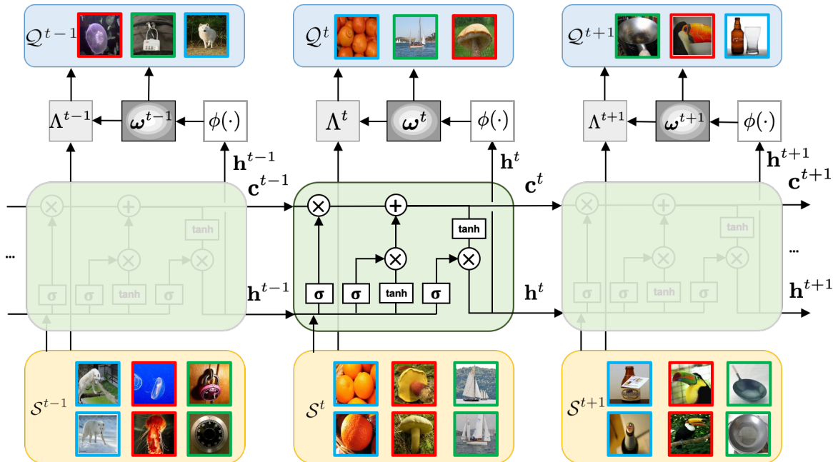
Figure 1. The learning framework of our meta variational random features (MetaVRF). The meta-learner employs an LSTM-based inference network ( ) to infer the spectral distribution over \Lambda^t , the kernel from the support set S^t of the current task t , and the outputs \mathbf{h}^{t-1} and \mathbf{c}^{t-1} of the previous task. During the learning process, the cell state in the LSTM is deployed to accumulate the shared knowledge through experiencing a set of prior tasks. The remember and forget gates in the LSTM episodically refine the cell state by absorbing information from each experienced task. For each individual task, the task-specific information extracted from its support set is combined with distilled information from the previous tasks to infer the adaptive spectral distribution of the kernels.
