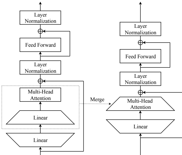
Figure 2. Adding linear transformation pairs into a thin BERT model. Left panel: a pair of linear transformation are inserted between any two adjacent transformer blocks. Right Panel: the linear transformation right next to the multi-head attention module (see the dashed box in the left panel) is merged before the training in the second stage, i.e., the stage of narrow learning, while the remaining linear transformation will be merged after fine-tuning when the whole training procedure is done. Thus, finally, the trained model has the exact same network architecture and number of parameters as the original thin model.
