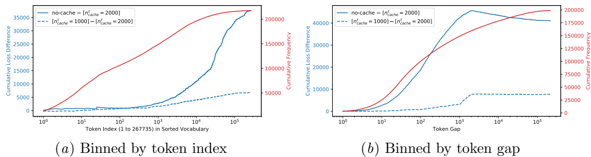
Figure 3: Blue: cumulative sum over the binned validation loss-difference between n_{\text{cache}}^t \in \{\text{no-cache}, 1000\} and n_{\text{cache}}^t = 2000 . Red: cumulative bin size for comparison. If the loss-difference were equally distributed across all tokens, the cumulative loss-difference would exactly match the cumulative bin size. All experiments are performed with C = 97 , Hebbian softmax, and no compression techniques.
