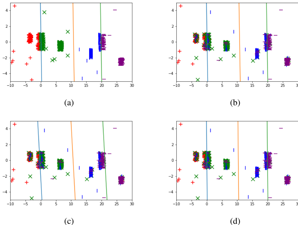
Figure 3: Results of different algorithms on Synthetic Dataset. (a) True classifier on clean data, (b) True classifier shown on noisy labels, (c) Classifier trained on noisy labels using l , (d) Classifier trained on noisy labels using \tilde{l} with known noise rates
