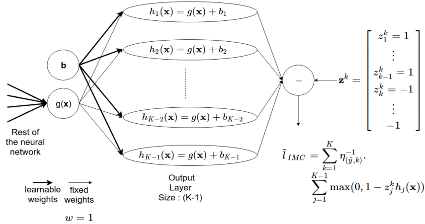
Figure 2: Neural network for robust ordinal regression using \tilde{l}_{IMC} .
