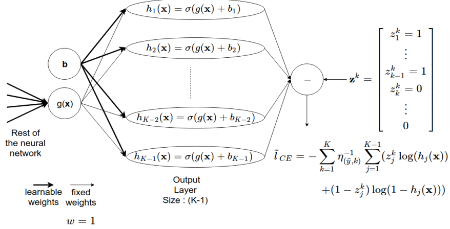
Figure 1: Neural network for robust ordinal regression based on \tilde{l}_{CE} .
