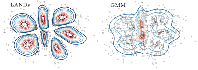
Figure 3: Using the samples in \mathcal{Z} generated from the proposed q(\mathbf{z}) we fit a mixture of LANDs and a GMM. Thus, we can capture the true underlying structure of the data manifold in the latent space of a GAN.
