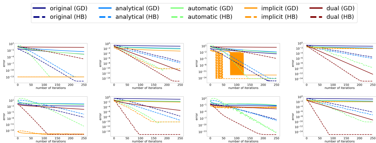
Figure 3: Error plots for problems listed in Section 3 for two more values of P , i.e., 70 (top row) and 30 (bottom row).
