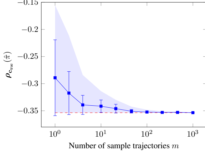
Figure 2. Performance of learned policies for a 16-by-16 gridworld environment. The dashed line shows \rho_{c_{\text{true}}}(\pi_E) . The error bars show the mean and standard deviation over 20 runs and the shaded area provides bounds for the computed policies.
