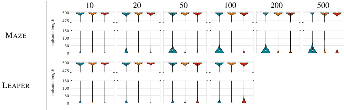
Figure S2: Density plots of performance on the test set (1000 unseen levels) after different number of training levels for the MAZE and LEAPER environments, the white point denotes the median performance on the test set.
