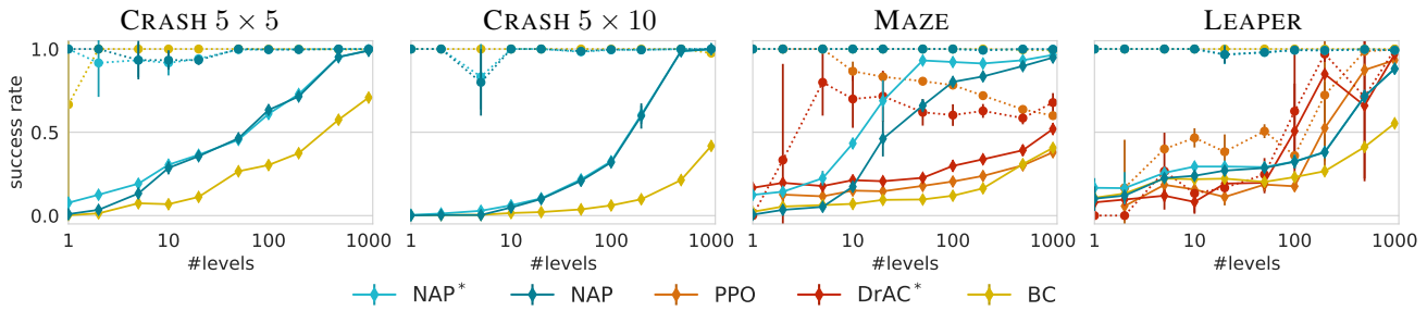
Figure S1: The dotted lines denote the training performance of the methods. We observe that the behavior cloning baseline and NAP have fitted the training set almost perfectly.
