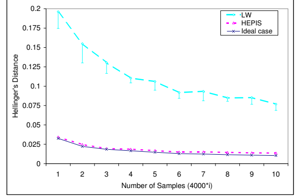
Figure 7: Error curves of LW and HEPIS-BN on the dynamic emission network.
