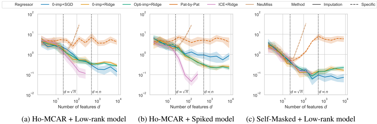
Figure 1. Risk w.r.t. the input dimension (evaluated on 10^4 test samples) when 50% of the input data is missing. The y -axis corresponds to R_{\text{mis}}(f) - R^* = \mathbb{E}[(Y - f(X_{\text{imp}}, P))^2] - \sigma^2 . The averaged risk is depicted over 10 repetitions within a 95% confidence interval.
