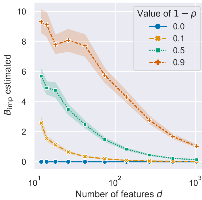
Figure 2. Estimated imputation bias with n = 10000 observations in a low rank setting ( r = 5 ).
