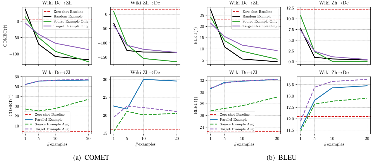
Figure 8: Results for few-shot prompting with monolingual data on Wiki Ablation sets for De \leftrightarrow Zh .
