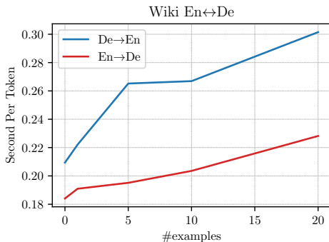
Figure 2: Inference time per token in seconds for zero/few-shot prompting on Wiki En-De Ablation sets. Numbers are averaged over 3 runs with 3 distinct demonstrations on 4 A100-40G GPUs.
