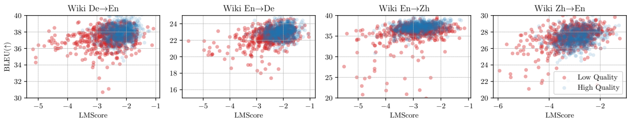
Figure 6: Scatter plotting between BLEU and LMScore for 1-shot prompting on Wiki De↔En, En↔Zh Ablation sets.
