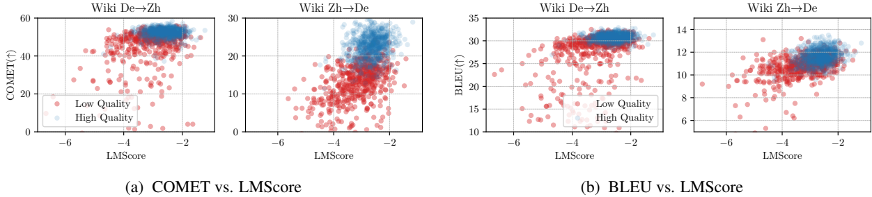
Figure 7: Scatter plotting between COMET/BLEU and LMScore for 1-shot prompting on Wiki De↔Zh Ablation sets.
