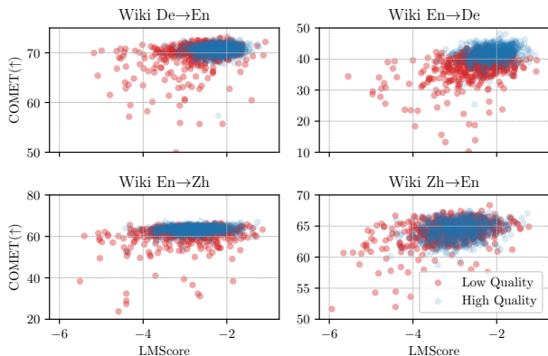
Figure 3: Visualization between COMET and LMScore for 1-shot prompting on Wiki Ablation sets. While correlations are significant, data points are scattered like clouds.
