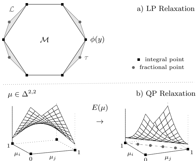
Figure 1. Tractable approximations of the MAP problem. In the exact LP and QP formulations, solutions are integral and occur at corner points of the constraint set. a) In the LP relaxation, corner points need no longer be integral. b) In the convex QP relaxation, convexification of the energy can lead to additional solutions in the interior.
