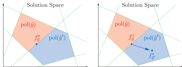
Figure 3. (Left) The conditionally optimal solution f_{\hat{y}}^* is at a boundary of the convex polytope \text{pol}(\hat{y}) , which indicates that f_{\hat{y}}^* is not a local optimal solution (see Theorem 4). By flipping some labels in \hat{y} , another convex polytope (blue one) is defined, and f_{\hat{y}}^* is feasible also in this polytope. (Right) According to Theorem 5, f_{\hat{y}}^* is not conditionally optimal in the adjacent polytope \text{pol}(\hat{y}') , where \hat{y}' is defined by (10). The conditionally optimal solution f_{\hat{y}'}^* would be elsewhere in the blue polytope, and it is guaranteed to be strictly better than f_{\hat{y}}^* .
