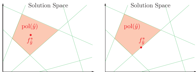
Figure 2. Illustration of S^3VM local optimal solutions. Each green line in the solution space represents f(x_i) = 0, i \in \mathcal{U} . If predicted labels \hat{y} is given, a convex polytope \text{pol}(\hat{y}) is defined by a set of these green lines. (Left) The conditionally optimal solution f_{\hat{y}}^* in \text{pol}(\hat{y}) is local optimal because it is located in the strict interior of \text{pol}(\hat{y}) . (Right) On the other hand, f_{\hat{y}}^* is not local optimal because it is at the boundary of \text{pol}(\hat{y}) .
