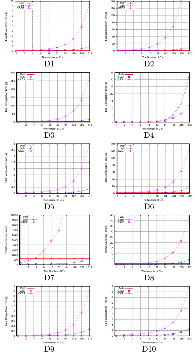
Figure 6. Total computation time for computing a sequence of solutions for different C^* s. The horizontal axis indicates the number of annealing steps in S^3VM^{\text{light}} and the number of candidates of C^* in CCCP. Note that the total computation time of S^3VM^{\text{path}} does not depend on the number of C^* s because it computes the entire path of solutions with an infinitesimal resolution.
