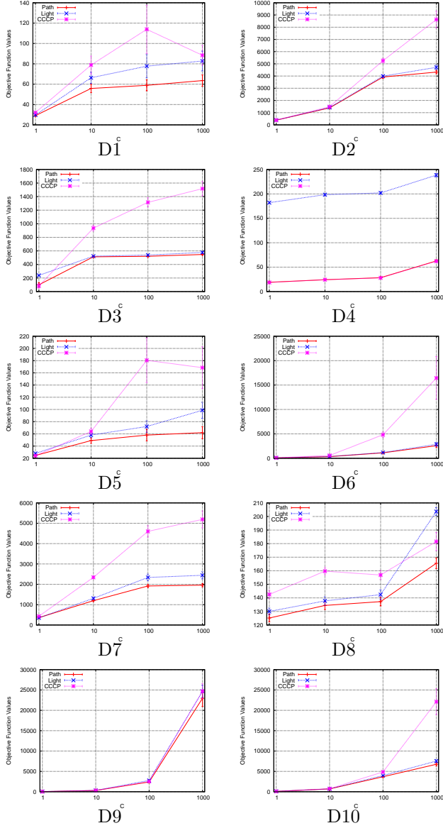
Figure 5. Objective function values J(f, \hat{y}) on labeled and unlabeled training instances at C^* = C for S^3VM^{\text{path}} , S^3VM^{\text{light}} , and CCCP. Smaller values means that better local optimal solutions are found.
