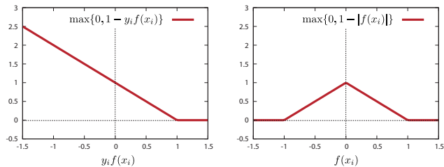
Figure 1. Loss functions for S^3VM . Left: Convex hinge loss for labeled instances. Right: Non-convex symmetric hinge loss for unlabeled instances.
