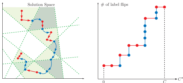
Figure 4. A Schematic illustration of the behavior of the S^3VM^{\text{path}} algorithm. (Left) S^3VM solution space consists of a number of convex polytopes, each characterized by the predicted label \hat{y} . As long as the conditionally optimal solution (see Definition 1) is in the strict interior of the current polytope, we can use a conventional parametric programming (a.k.a. regularization path following) to keep track of a local optimal solution path (the CP step: Red arrows and points). However, once the solution reaches a boundary of the current convex polytope, the algorithm jumps to the conditionally optimal solution in the adjacent polytope (the DJ step: Blue arrows and points). (Right) Illustration of how C^* is increased in S^3VM^{\text{path}} . We continuously increase C^* from 0 to C while we are computing a local optimal solution path (CP step: red lines and points). Once we reaches a boundary of the polytope, we fix C^* until we find a local optimal solution at that C^* (DJ step: blue lines and points).
