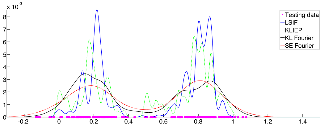
Figure 1: Plot of the learned weight functions \hat{w} for a 1D toy example. Regions of low test data (magenta) density imply small weights while high density regions imply large weights. KLIEP (green) and uLSIF (blue) compute much more volatile weight functions than the Fourier methods. Total variation Fourier was omitted in this plot for clarity of the diagram and due to similarity to the other shown Fourier results.
