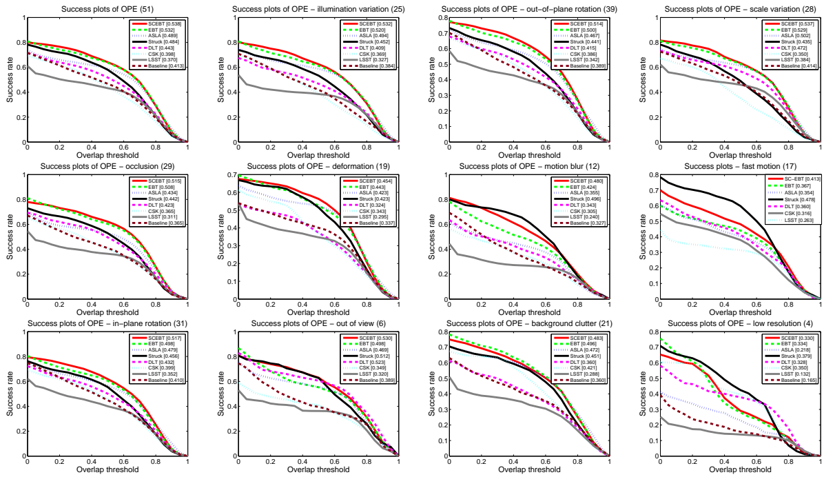
Figure 2: ROC curves based on the overlap rate metric for different categories of test sequences. The title of the subfigure for each category shows the number of video sequences (in brackets) in that category.
