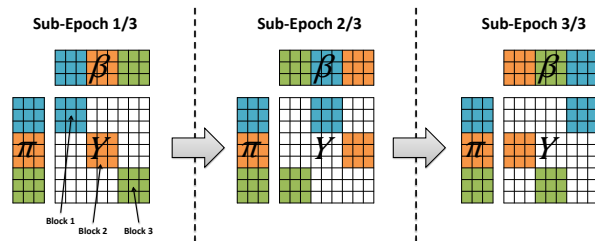
Figure 1: Partitioning strategy for data Y , model variables \pi , and parameters \beta . We show one epoch broken into multiple sub-epochs (3 in this case). Each sub-epoch is further divided into (colored) blocks, such that the data Y_{i,j} (with its associated variables \pi_{i,\cdot} and parameters \beta_{\cdot,j} ) from one block do not share rows/columns with data Y_{a,b} from another block. Taken together, all blocks from all sub-epochs cover every element of Y, \pi, \beta .
