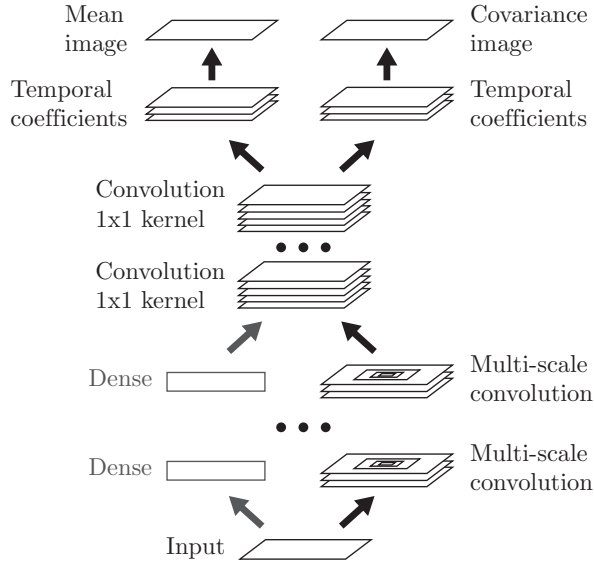
Figure D.1. Network architecture for mean function f_{\mu}(\mathbf{x}^{(t)}, t) and covariance function f_{\Sigma}(\mathbf{x}^{(t)}, t) , for experiments in Section 3.2. The input image \mathbf{x}^{(t)} passes through several layers of multi-scale convolution (Section D.2.1). It then passes through several convolutional layers with 1 \times 1 kernels. This is equivalent to a dense transformation performed on each pixel. A linear transformation generates coefficients for readout of both mean \mu^{(t)} and covariance \Sigma^{(t)} for each pixel. Finally, a time dependent readout function converts those coefficients into mean and covariance images, as described in Section D.2.1. For CIFAR-10 a dense (or fully connected) pathway was used in parallel to the multi-scale convolutional pathway. For MNIST, the dense pathway was used to the exclusion of the multi-scale convolutional pathway.
