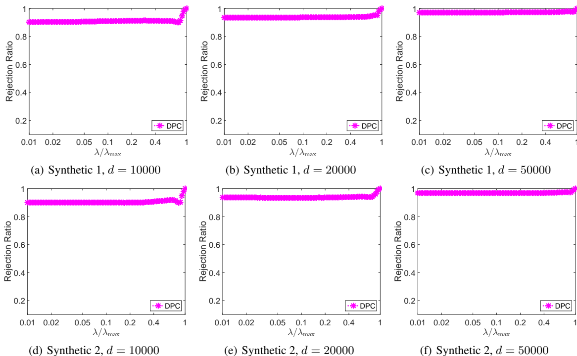
Figure 1. Rejection ratios of DPC on two synthetic data sets with different feature dimensions.
