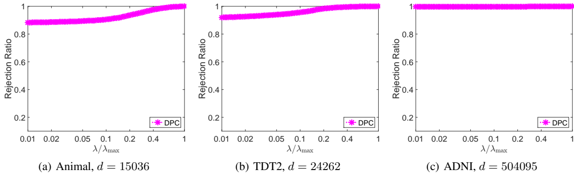
Figure 2. Rejection ratios of DPC on three real data sets.
