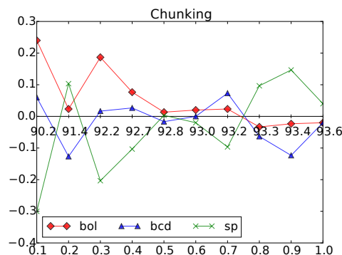
Figure 3. Performances on chunking. x-axis represents the proportion of training set. y-axis is the F1-value.
