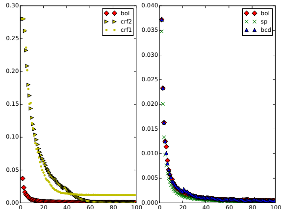
Figure 2. Convergence speeds on the pku data set. x-axis is the number of iterations, y-axis is the label error rate. “bol” converges much faster than CRFs, and it is slightly slower than “sp”.
