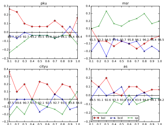
Figure 1. Performances on word segmentation. x-axis is the proportion of training set. The horizontal line y = 0 is the average F1 value among algorithms, and y-axis is the offset against average.
