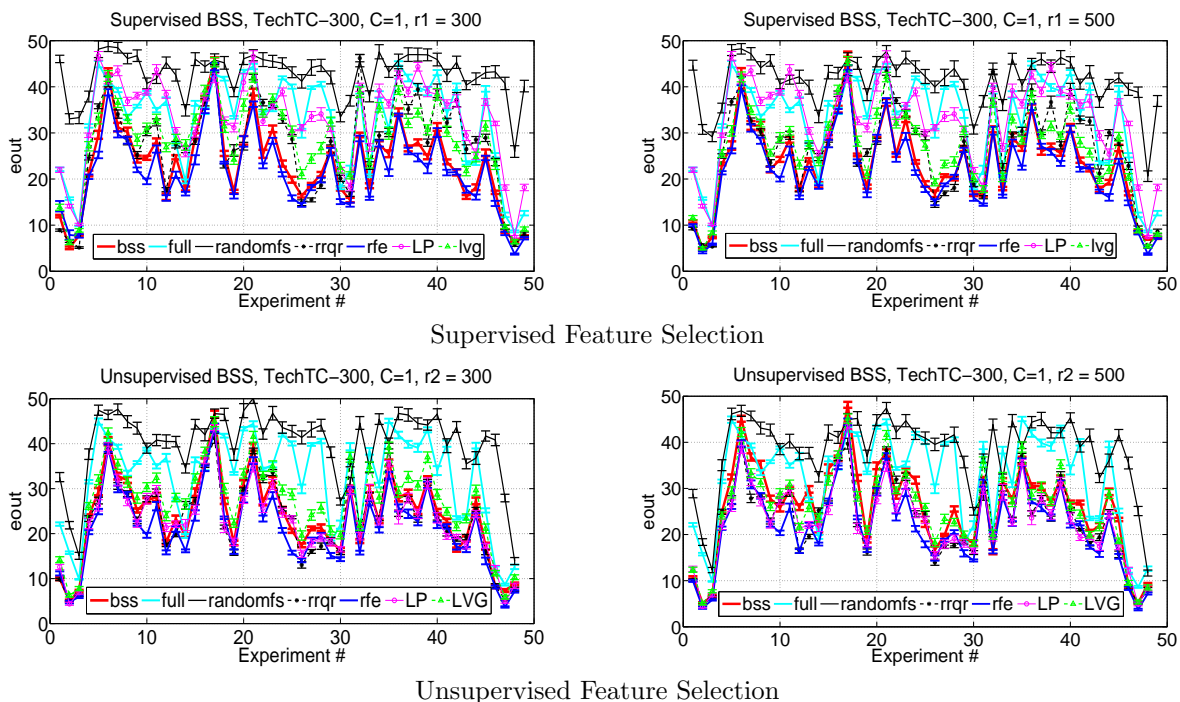
Figure 1: Plots of out-of-sample error (eout) of Supervised and Unsupervised BSS and leverage-score compared with other methods for 49 TechTC-300 documents averaged over ten ten-fold cross validation experiments. Vertical bars represent standard deviation.
