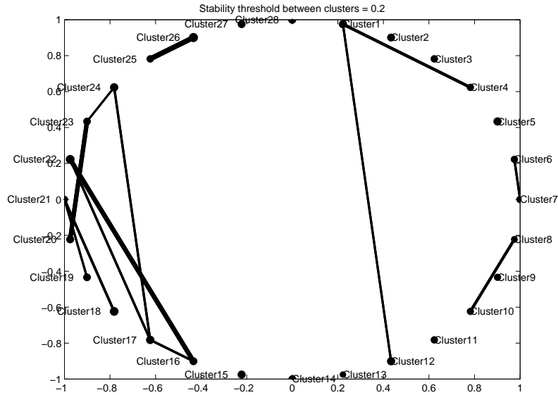
Figure 4: Graph representing clusters and their connections. The thickness of each link is proportional to the value S_{inter} . Isolated clusters correspond to high S_{intra} values.
