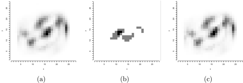
Figure 7: Variable importance for MNIST dataset: (a) average, (b) 5% quantile, (c) 95% quantile. Black corresponds to the maximum importance.
