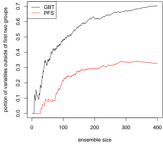
Figure 4: The number of variables outside the first two groups selected for splits normalized on ensemble size.
