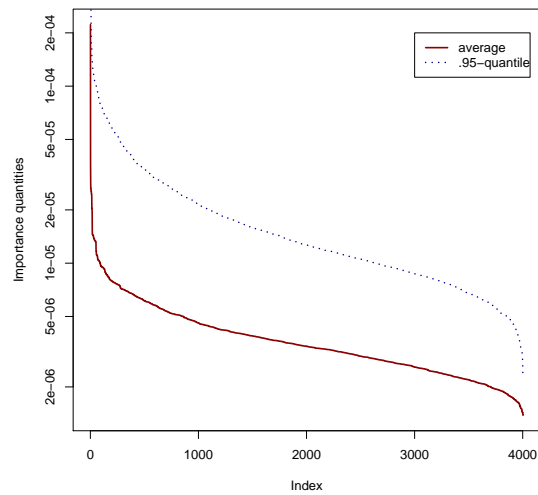
Figure 6: The distribution of variable importance for UCR datasets.
