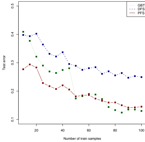
Figure 5: Linear Regression problem: the dependence of test error on the number of samples.
