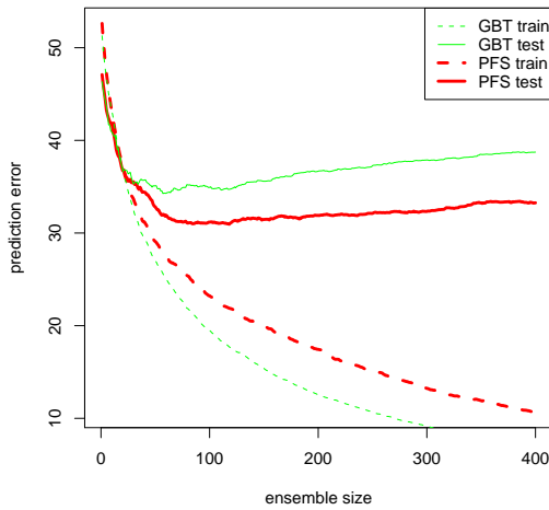
Figure 3: GBT and PFS stumps training and test error versus ensemble size.
