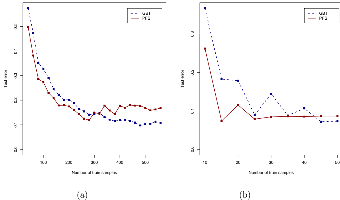
Figure 9: The dependence of test error on the training set size for UCR datasets: (a) FaceAll, (b) GunPoint
