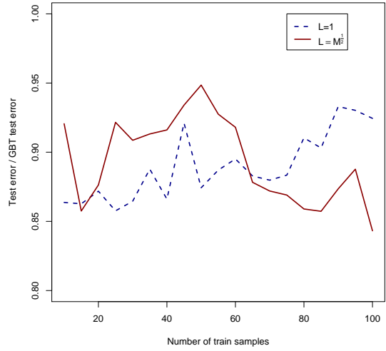
Figure 2: PFS test error normalized on GBT test error vs. training set size.
