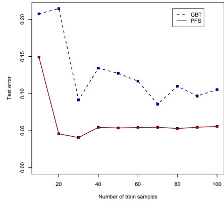
Figure 8: The dependence of test error on the number of training samples for MNIST problem 1 vs 3.
