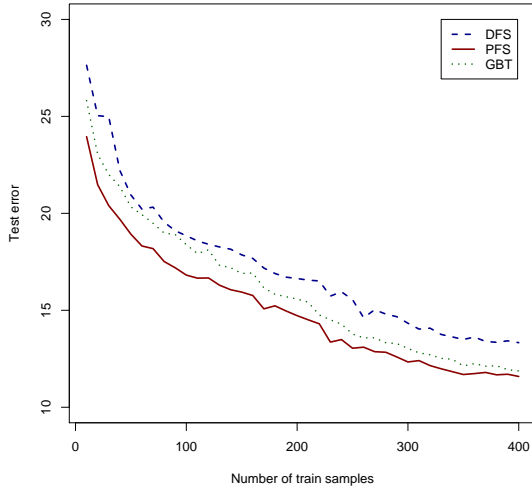
Figure 1: Test error vs. training set size.
