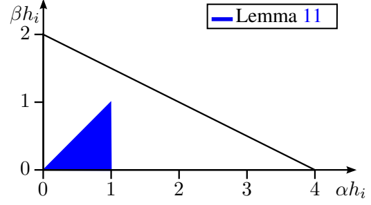
Figure 12: Validity of Lemma 11
