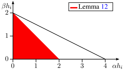
Figure 13: Validity of Lemma 12
