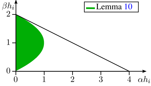
Figure 11: Validity of Lemma 10
