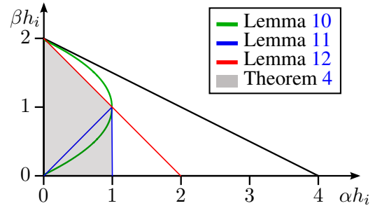
Figure 14: Area of Theorem 4
