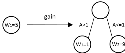
Figure 2: Tree Splitting
