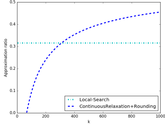
Figure 5. Approximation guarantees of the two algorithms as a function of the second stage constraint k .
