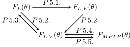
Figure 3: Monotone transformations between different representations.
