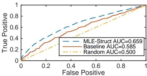
(a) ROC curves for roommate matching of our algorithm and a constant baseline.
