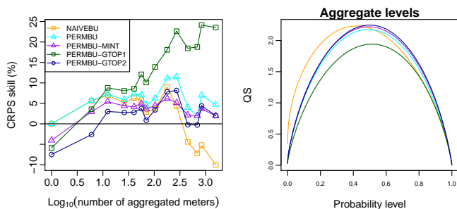
Figure 4. CRPS skill for different aggregations and average QS of all aggregate series. A positive/negative CRPS skill gives the percentage of decrease/increase in CRPS with respect to the base forecasts. Higher skill score and lower QS are better.
