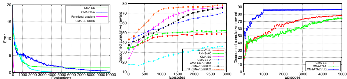
Figure 3: Results for (left) 2D synthetic domain, (center) the inverted pendulum domain; (right) Double-link
