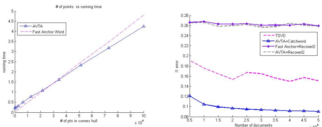
(c) Running time (secs) of computing vertices of simplex (d) \ell_1 error in the semi-synthetic dataset.
