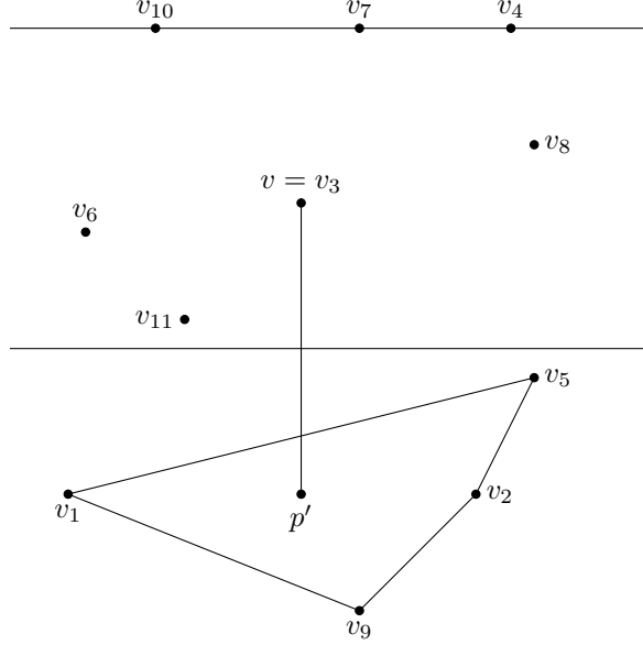
Figure 3: An example where \widehat{S} = \{v_1, v_9, v_2, v_5\} , then v = v_3 is randomly selected from S \setminus \widehat{S} and is tested if it lies in \text{conv}(\widehat{S}) . A witness p' is found. Then using c' - v - p' the set S' = \{v_4, v_7, v_{10}\} is computed and one of vertices of \text{conv}(S') , i.e. v_4 or v_{10} is selected for inclusion in \widehat{S} .
