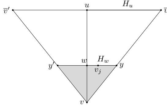
Figure 4: Given v \in \bar{S} , u is its closet point in \text{conv}(\bar{S} \setminus \{v\}) . \bar{v}, \bar{v}' \in \bar{S} are vertices of \text{conv}(S) lying on H_u , the orthogonal hyperplane to line segment uv at u . u is a convex combination of these vertices. Moving H_u parallel to itself toward v , it intersects the line segment uv at a unique point w lying on a facet of \text{conv}(S \setminus \{v\}) . Thus interior of shaded region contains no point of S .
