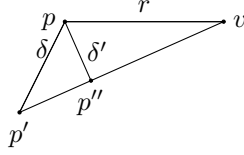
Figure 2: Reduction of gaps \delta = \|p' - p\| by using a p -pivot v , \delta' = \|p'' - p\| .
