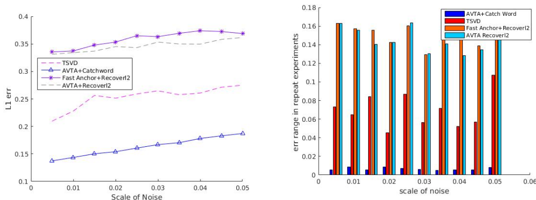
(e) \ell_1 error in the perturbed semi-synthetic dataset. (f) Range of the \ell_1 error over 10 runs on the noisy semi-synthetic dataset.
