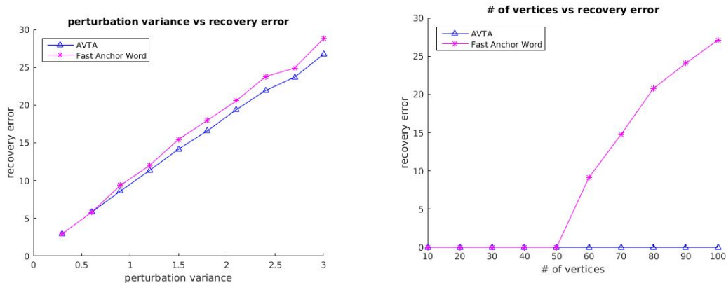
(a) Recovery error-computing vertices (simplex case) (b) Recovery error-computing vertices (general convex hull)
