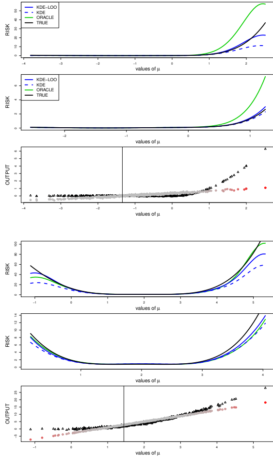
Figure 3: Top/middle : graph of R_{\mu,\Gamma}(g) for TRUE, KDE-LOO, KDE and ORACLE, when \mu lives in the whole range of x_{i,1} (top) and zooming around the mean of x_{i,1} . Bottom : outputs y_i and predicted values g(x_{i,1}) versus x_{i,1} . Red and grey colors reflects large and small values of KDE-LOO. In the right, a = -1 . In the left a = 2 . The signal-noise quotient is 0.1.
