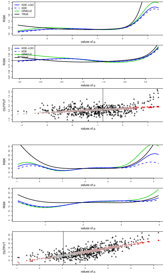
Figure 5: Top/middle : graph of R_{\mu,\Gamma}(g) for TRUE, KDE-LOO, KDE and ORACLE, when \mu lives in the whole range of x_{i,1} (top) and zooming around the mean of x_{i,1} . Bottom : outputs y_i and predicted values g(x_{i,1}) versus x_{i,1} . Red and grey colors reflects large and small values of KDE-LOO. In the right, a = -1 . In the left a = 2 . The signal-noise quotient is 1.
