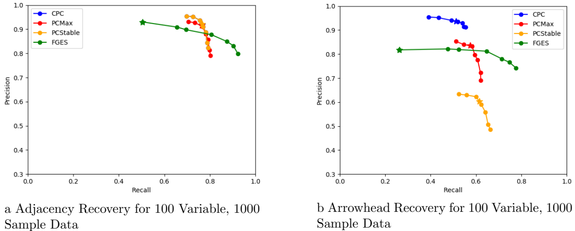
Figure 1: Precision-Recall Plots for 100 variable, 1000 sample, continuous datasets. The star refers to the average parameter values chosen by StARS. The CPC results are identical to the PC-Stable results in (a).
