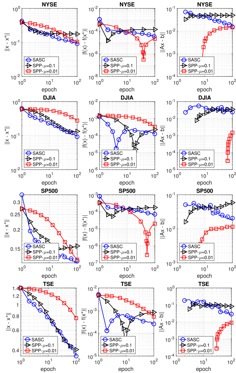
Figure 4. Performance of SASC and SPP on portfolio optimization for four different datasets
