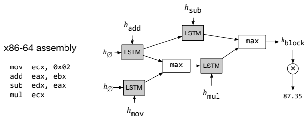
Figure 4. The DAG-RNN Architecture
