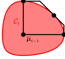
Figure 2. Illustration of Theorem 1: The confidence region C_t and the polymatroid defined by the submodular function A \mapsto \max_{\mu \in C_t - \bar{\mu}_{t-1}} \mathbf{e}_A^\top \mu .
