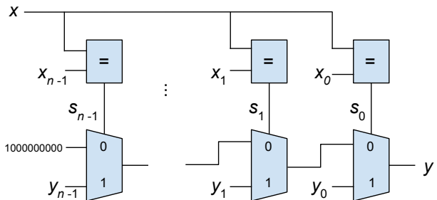
Figure 1: A circuit implementing a lookup table that memorizes the training examples (x_i, y_i) for 0 \leq i < n . We observe that in this extreme case of overfitting, there are signals in the circuit (the s_i ) that identify specific training examples. For e.g., s_0 is 1 only when x = x_0 and 0 for all other x_i (assuming the x_i are distinct). We say that 1 is a rare pattern for the signal s_0 . Based on this example, we propose that the occurrence of rare patterns during simulation of a training set through a model indicates overfitting, and in this work, we explore to what extent such rare patterns can be used to detect overfitting in more complex models such as neural networks and random forests.
