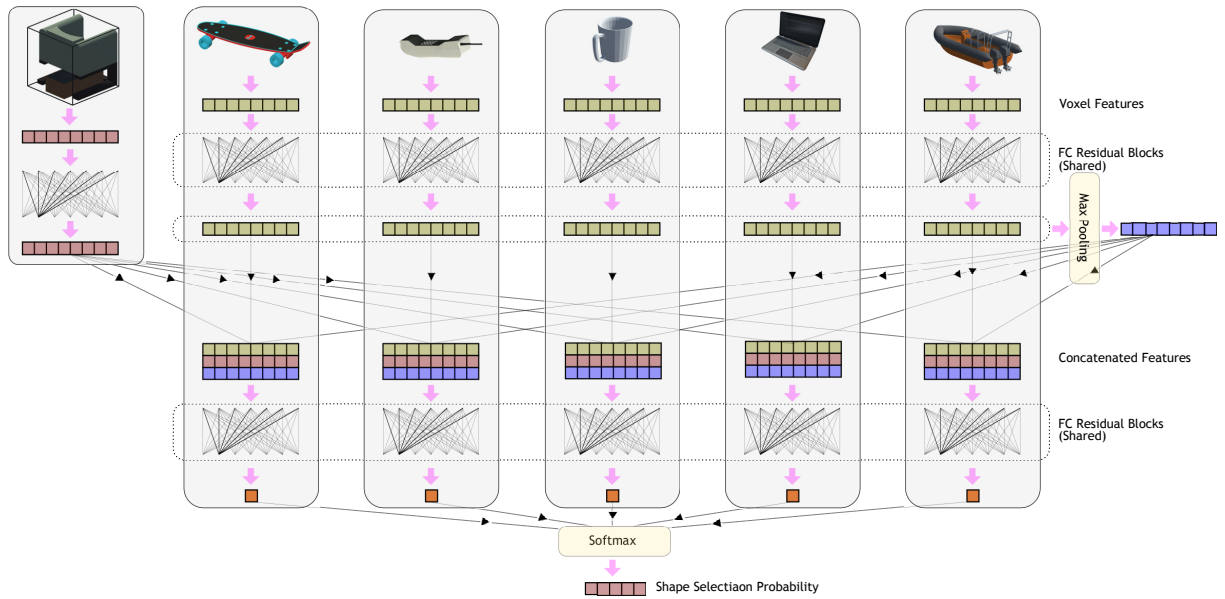
Figure 1: The proposed PackNN Neural Network for Shape Selection. Given the voxel representation of the candidate shapes and the box, PackNN outputs a probability distribution for selecting the next shape to be put in the box.
