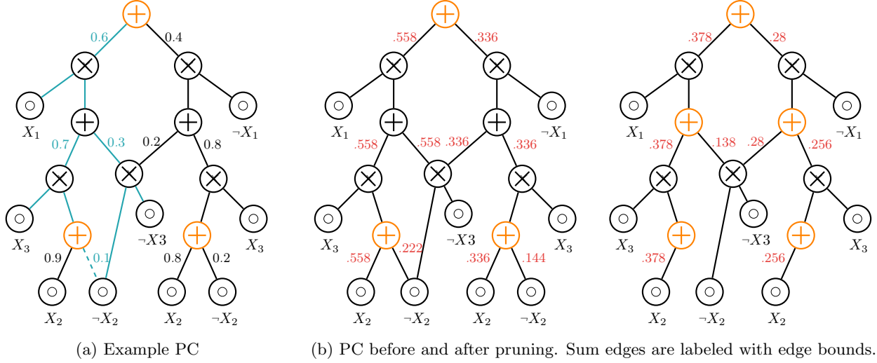
Figure 1: A smooth and decomposable PC over variables fX_1, X_2, X_3g . Orange sum nodes are \mathbf{Q} -deterministic for \mathbf{Q} = fX_1, X_2g ; blue edges form the sub-circuit for joint assignment \mathbf{q} = fX_1 = 1, X_2 = 0g .
