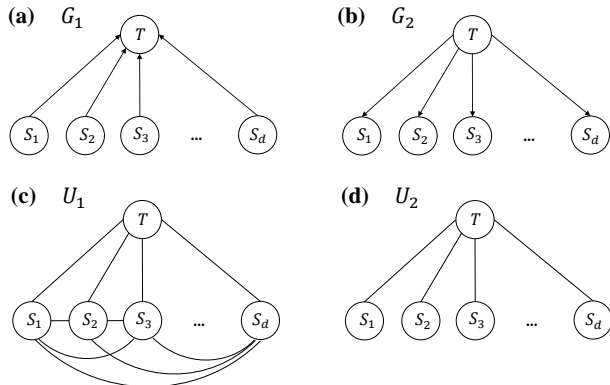
Figure 1: Illustrating examples to compare sample complexities for learning DAG and UG. (a) & (b) : The original DAGs; (c) & (d) : The UGs generated under equal variance condition by DAGs in (a) & (b) respectively.
