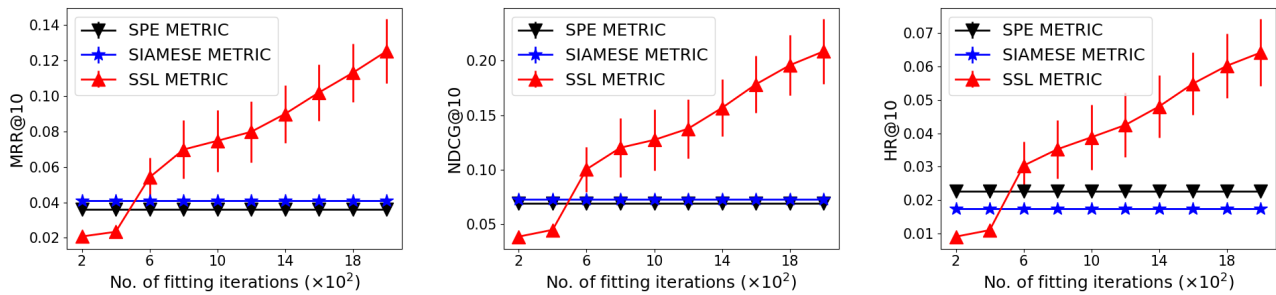
Figure 2: Plots of the averaged MRR, NDCG and HR measurements (over 5 independent SSL runs) of our SSL metric evaluated on YELP dataset. The performance of SPE and Siamese baselines were also included as references. These measurements however do not improve with more iterations as SPE and Siamese are non-SSL. Similar to our experiments with the MovieLens dataset, the MRR, NDCG and HR measurements are computed with respect to top-10 recommendation lists produced by the participating baselines on the same unseen test set.
