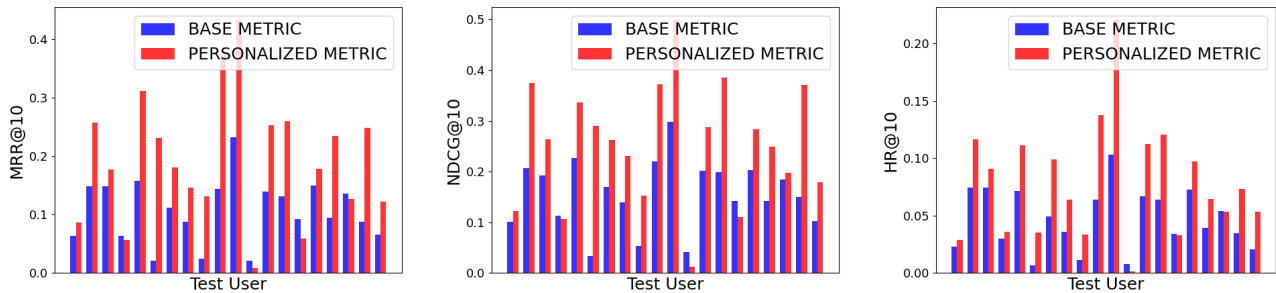
Figure 3: Bar charts of the individual MRR, NDCG and HR measurements of a set of 20 randomly sampled users with fewer than 200 interactions with items in the catalogue. Red (blue) columns reflect the measurement (MRR, NDCG and HR) of the personalized (base) SSL metric on those users.
