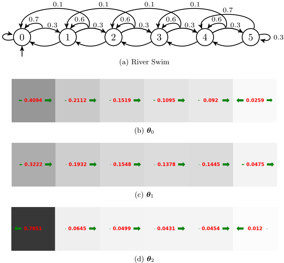
Figure 2: (a) Illustration of the River Swim CMP. (b, c, d) Heatmap visualization of the policies in the \sigma -compression \theta_k \in \Theta_\sigma for the River Swim domain. The background color and the label denote the state probability, the green arrows represent the policy in the state.
