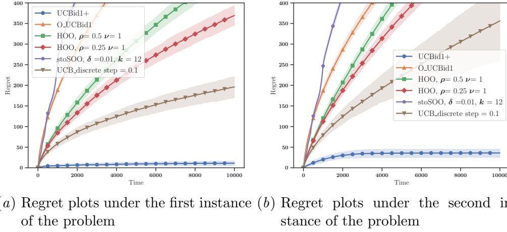
Figure 5: Regret plots for unknown F
