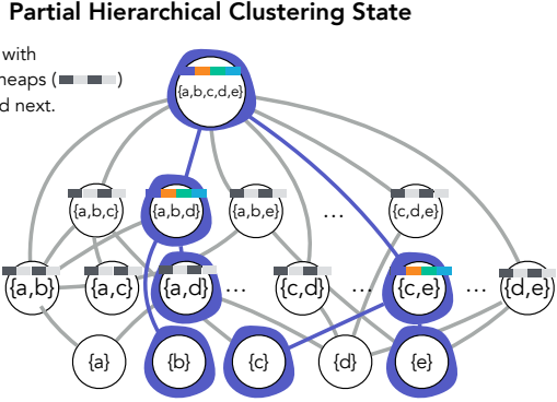
Figure 4: State Space A state (i.e., a partial hierarchical clustering) is compactly encoded as paths in the trellis structured, discovered by following the root-to-leaf pointers.
