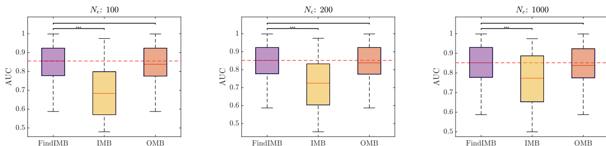
Figure 4: Boxplots of areas under the ROC curve for predicting Y_x using (a) FindIMB (b) IMB and (c) OMB. Data were simulated from random DAGs with 40 observed and 20 latent variables. D_o included 10,000 samples, and D_e included 100 (left), 200 (middle) or 1000 (right) samples. Black asterisks denote statistical significance, assessed with the Wilcoxon signed-rank test. Three stars correspond to p < 0.001 , no stars denote non-significance.
