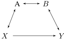
Figure 1: An example SMCM. \{X, A, B\} is the Markov boundary of Y in \mathcal{G}_{\bar{X}} . P(Y|do(X), A, B) is not identifiable from the observational distribution P , but P(Y|do(X), A) and P(Y|do(X), B) are. \{X, B\} is the causal Markov boundary for Y_X .
