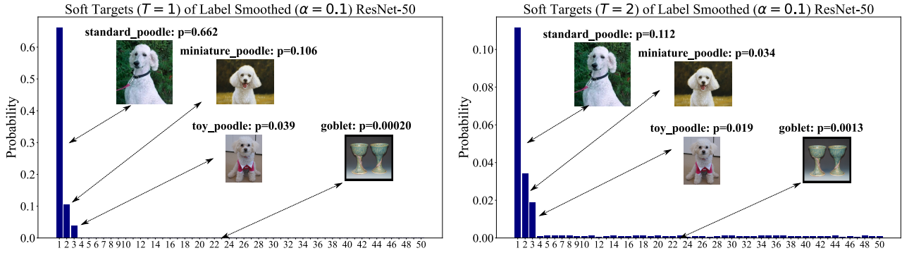
Figure 2. Soft output of the LS-trained ResNet-50 teacher ( \alpha = 0.1 ) same as the one in Figure 1. Left: soft output at T = 1 ; Right: soft output at T = 2 . The figures show the average of the soft outputs for 1300 training standard_poodle samples. Index 1 is the soft output for the standard_poodle class, i.e. p_k^t(T) . Index 2 and 3 are the soft outputs for the semantically similar classes miniature_poodle and toy_poodle respectively, i.e. p_{ml}^t(T) . The rest are soft outputs of randomly-chosen semantically dissimilar classes, i.e. p_{ms}^t(T) . Note that an increase of T brings p_{ml}^t(T) closer to p_k^t(T) . Therefore, soft targets at an increased T encourage student to learn penultimate representations closer to semantically similar class ml , which are miniature_poodle and toy_poodle in this case. Therefore, in Figure 1 Observation 3 , standard_poodle activations has more overlapping with miniature_poodle when KD of T = 2 is used. Also, p_{ms}^t(T) remains negligible after T scaling, as shown in the figure. Furthermore, the figure of T = 1 (Left) suggests that even with LS probabilities of incorrect classes \bar{p}_{m,g}^t are not all the same, and information erasure is not perfect in practice. Therefore, the diffusion of penultimate representations is not isotropic.
