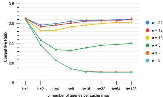
Figure 1. Average competitive ratio of AdaptiveQuery for different values of b and the error parameter \sigma .
