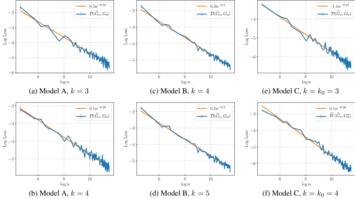
Figure 2. Log-log scale plots for the simulation results under Models A–C. For each model and sample size n , we compute the estimator \widehat{G}_n on 20 independent samples of size n . Its average discrepancy from the true mixing measure is plotted in blue, with error bars representing two empirical standard deviations. We additionally plot, in orange, the fitted linear regression line of these points, obtained using the method of least squares.
