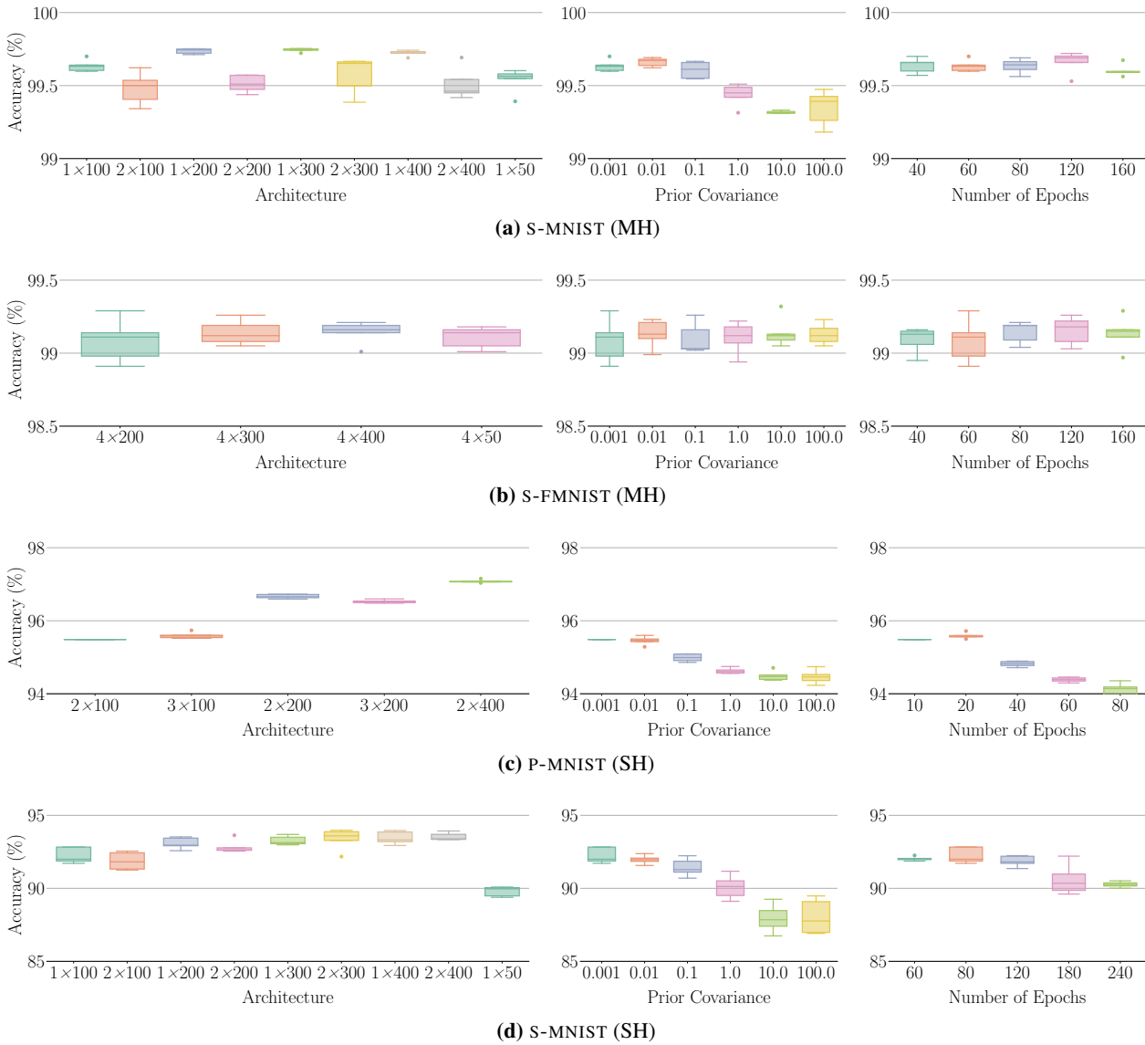
Figure 9. Effect of Neural-Network Size, First-Task Prior Covariance, and the Number of Training Epochs. We explore settings of neural-network size (e.g., 2 100 means a fully connected neural network with two hidden layers of size 100), initial prior covariance and number of training epochs for each task. To limit the computational resources required, we vary the values of one hyperparameter at a time instead of carrying out a full grid search.
