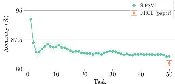
Figure 5. Predictive accuracies of S-FSVI and FRCL on sequential Omniglot. For S-FSVI, the accuracy shown at task t is the mean accuracy across all tasks up to that point (mean \pm one standard error as computed across five permutations of the task order). We were unable to reproduce the result reported in Titsias et al. (2020) using the authors’ code. However, we compare against the result from the paper (only the accuracy at task 50 is reported) here to provide a strong baseline.
