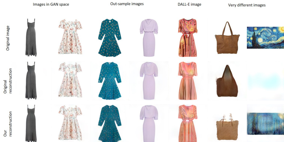
Figure 2: Example results of image embedding. The images in first row are the input images. The second row shows images found without using the pixel-level loss, and the third row shows images found using the pixel-level loss.
